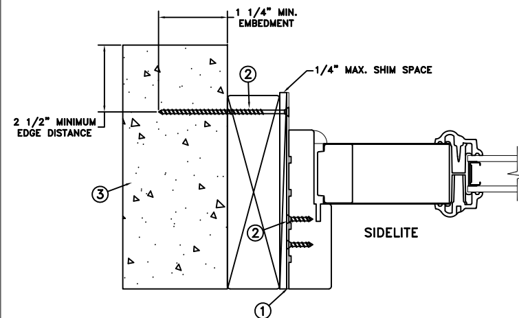
FRAME JAMB SECTIONS (TYP) HORIZONTAL SECTIONS
