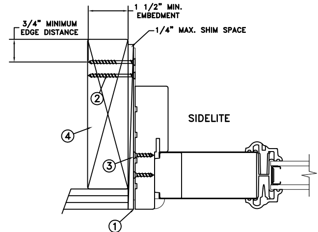
FRAME JAMB SECTIONS (TYP) HORIZONTAL SECTIONS
