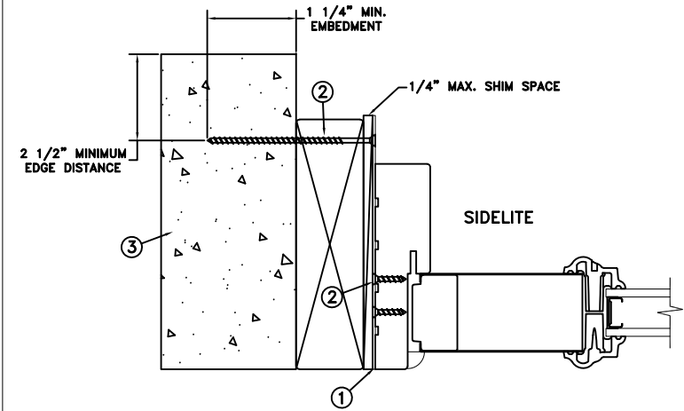
FRAME JAMB SECTIONS (TYP) HORIZONTAL SECTIONS
