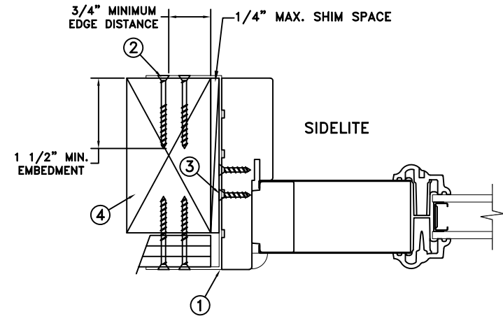
FRAME JAMB SECTIONS (TYP) HORIZONTAL SECTIONS
