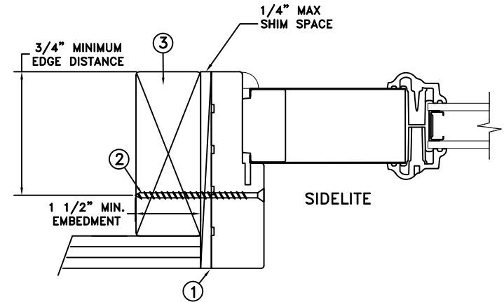
FRAME JAMB SECTIONS (TYP) HORIZONTAL SECTIONS
